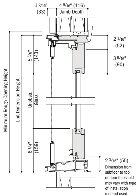
Vertical Section Active, Contemporary Panel, Gliding Insect Screen
