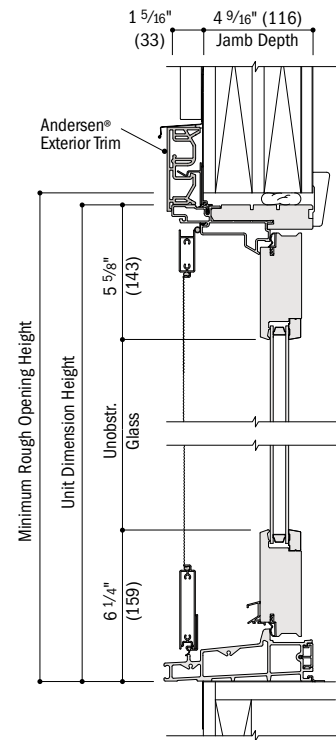
Vertical Section Active, Contemporary Panel, Hinged Insect Screen
