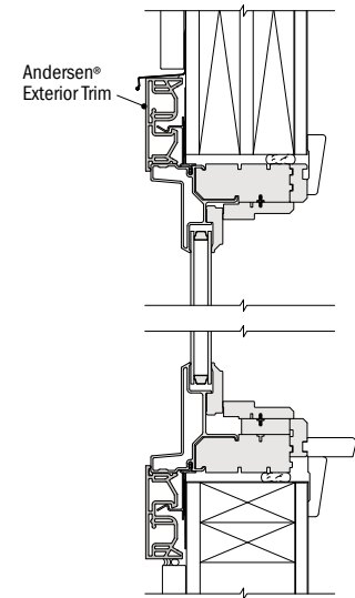
Vertical Section
