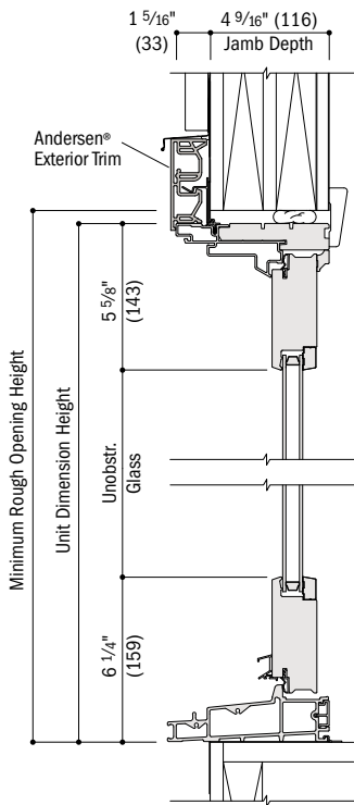
Vertical Section Stationary, Contemporary Panel
