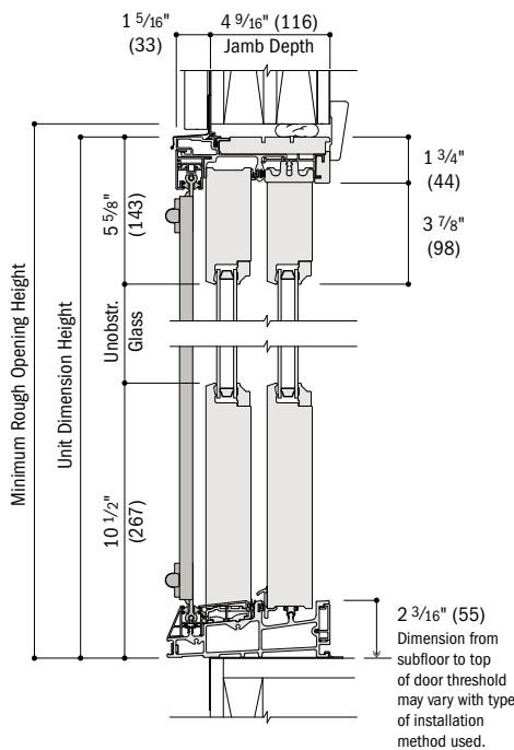
Vertical Section Operating, Traditional Panels, Retractable Insect Screen
