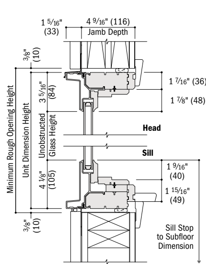
Vertical Section
